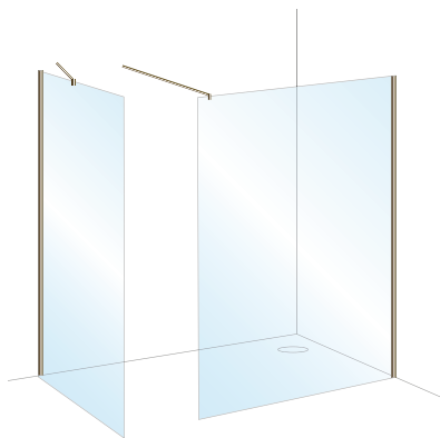
2 x Corner Panel 2 x Low Level Brace Kit
